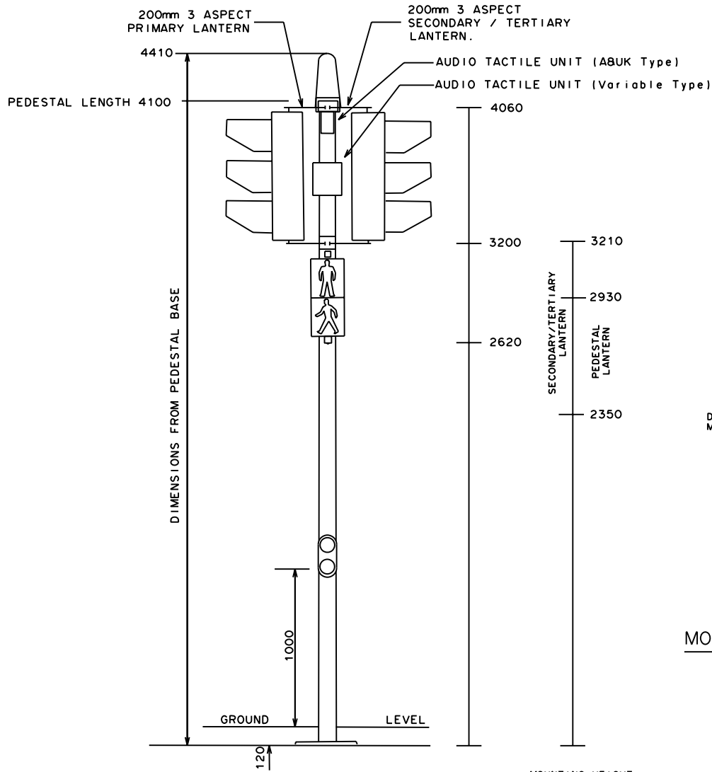
2B PEDESTAL
