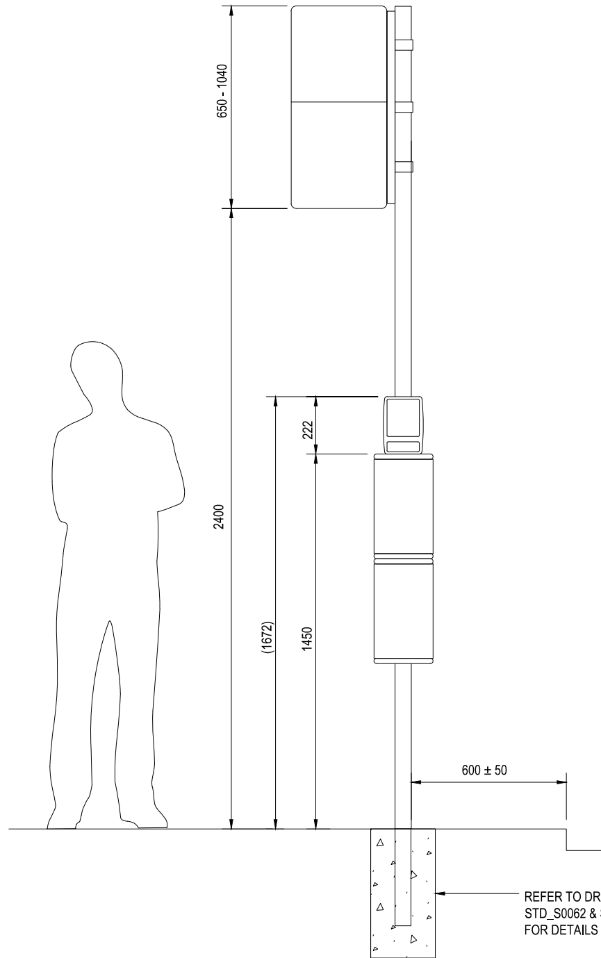
ELEVATION - SINGLE SIDED SCALE 1 : 20
