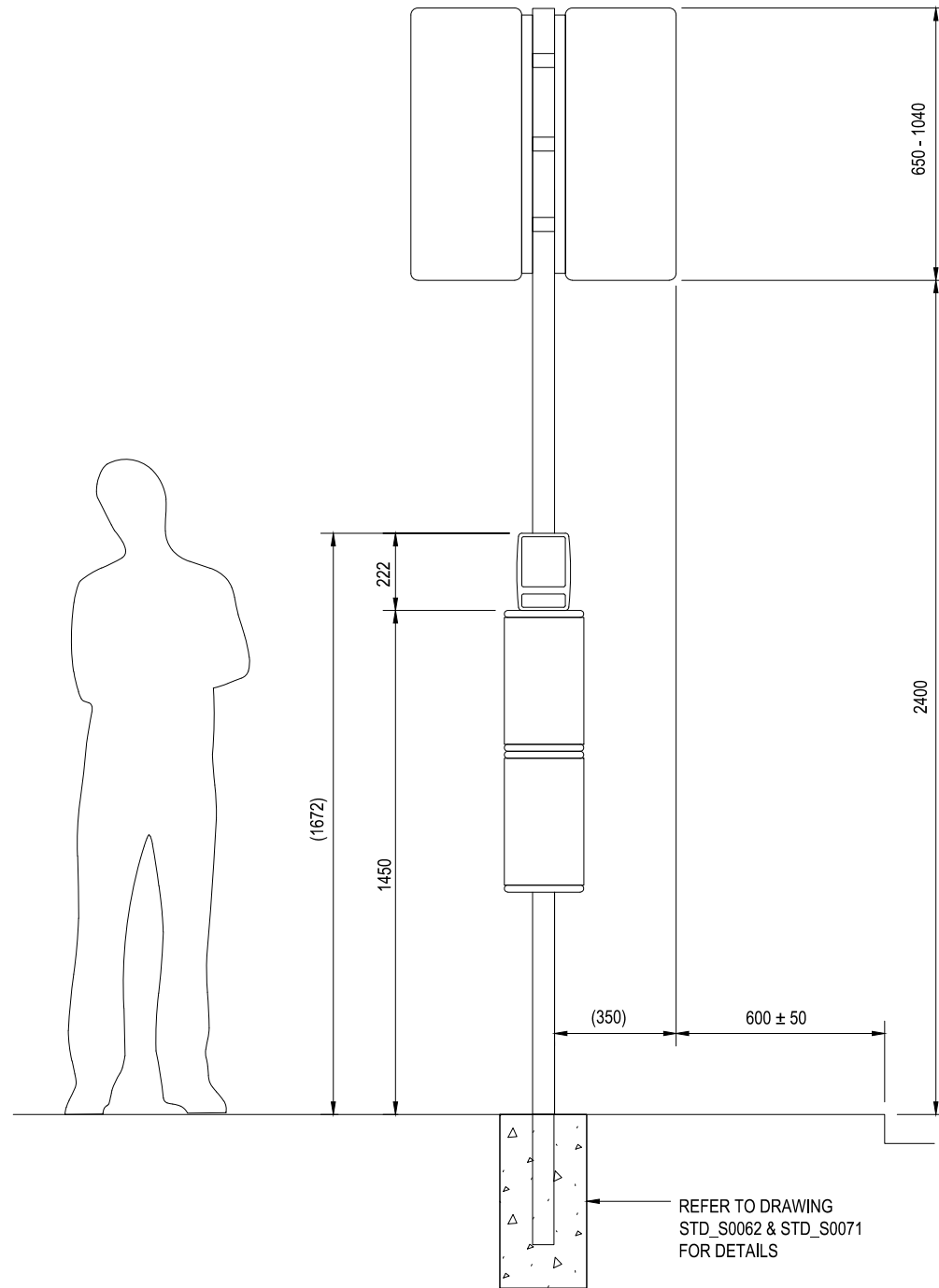
ELEVATION - DOUBLE SIDED SCALE 1 : 20
