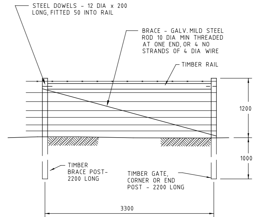
SINGLE STRAINER ASSEMBLY FOR USE AT GATEWAYS, ENDS, ANGLES, ETC.
